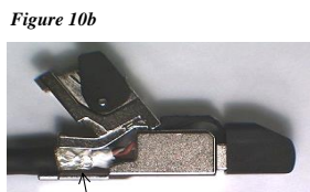
align shields under clamp
