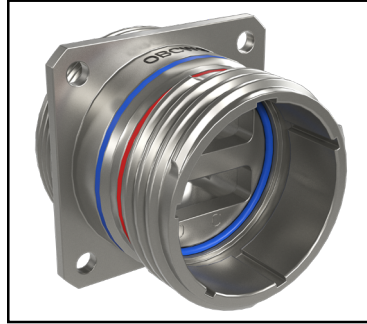
Flange Mount Shell - Electroless Nickel
