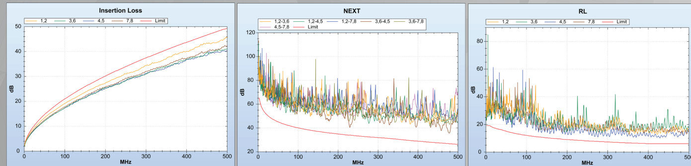
*E6A6824 electrical performance over 80M with 6.4dB of headroom
